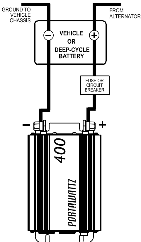
Figure 2 - Connection to a Battery
